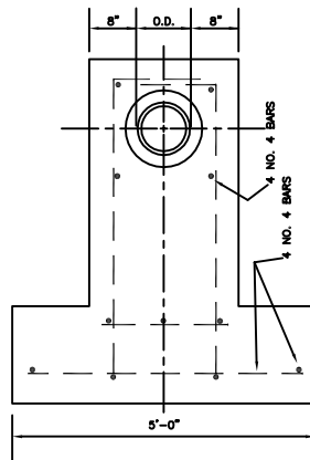
STANDARD CONCRETE PIER NOT TO SCALE
