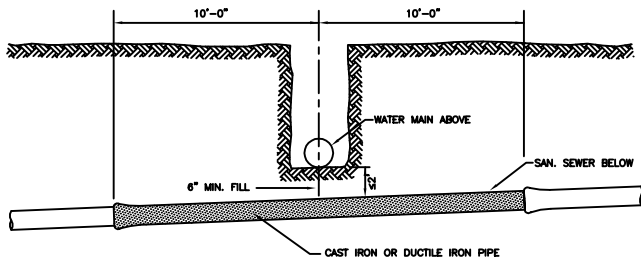
SANITARY SEWER CROSSING NOT TO SCALE
