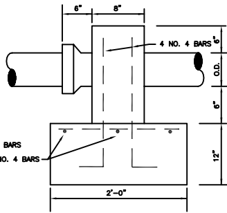
RESTRAINING COLLAR CONCRETE PIER NOT TO SCALE
