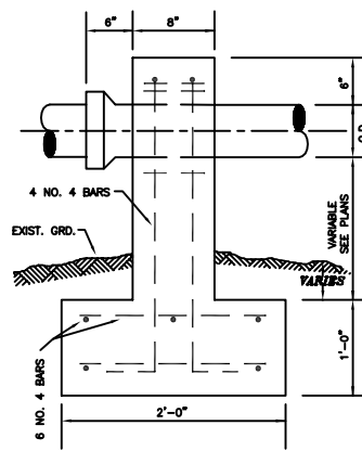
STANDARD CONCRETE PIER NOT TO SCALE
