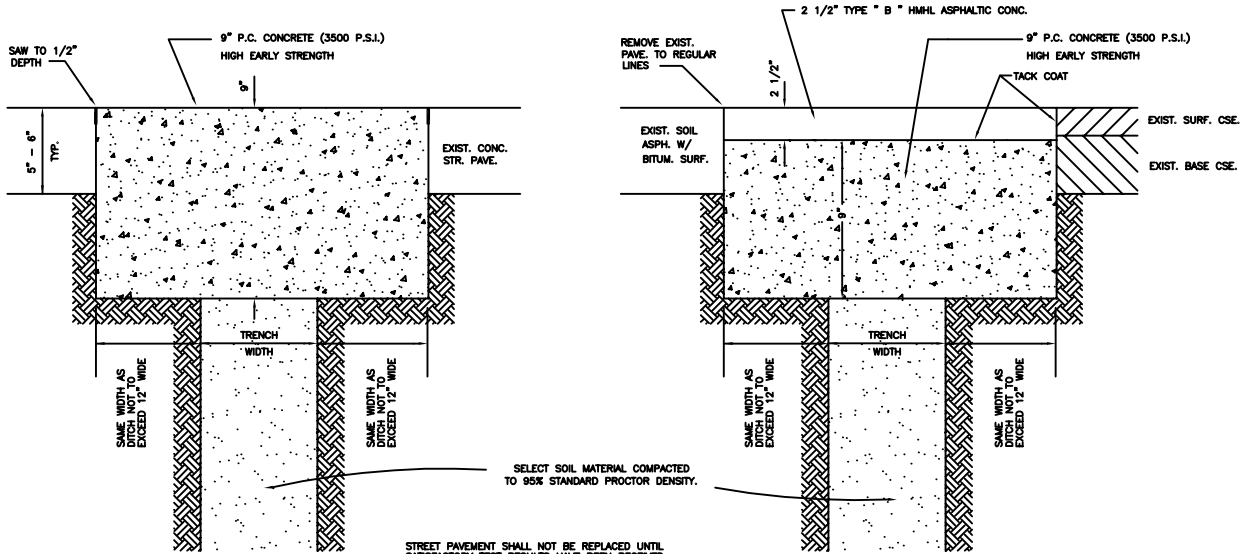
TYPICAL SECTION FOR REPLACEMENT OF P.C. CONCRETE STREET & ALLEY PAVEMENT
