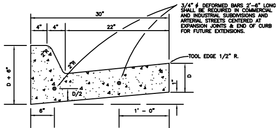
COMBINED CURB & GUTTER DETAIL
